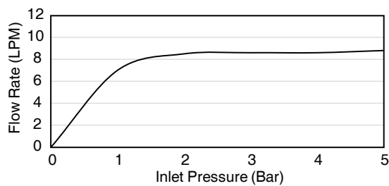
Flow Curve - Showerhead
