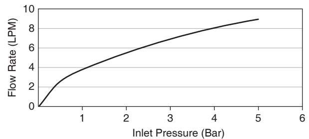
Flow Curve Handshower (K-76233X-CP)
