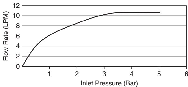
Flow Curve Showerhead (K-76233X-CP)
